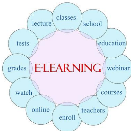
Figure 1 E-Learning concept
